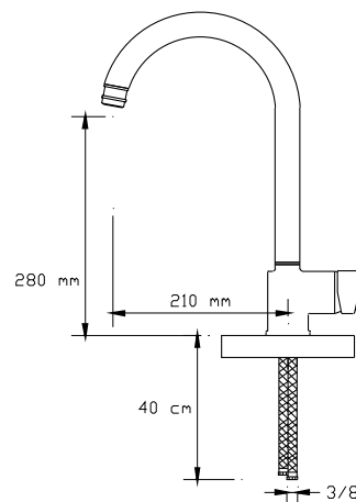
Sink Mixer With Pull-Out Spiral Spring Tap
