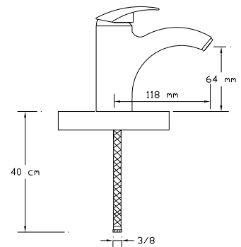
Basin Mixer Single Output
